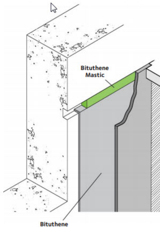
bituthene-mastic
