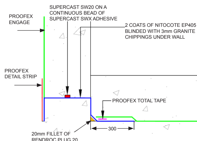
Typical application within a foundation concrete construction joint
