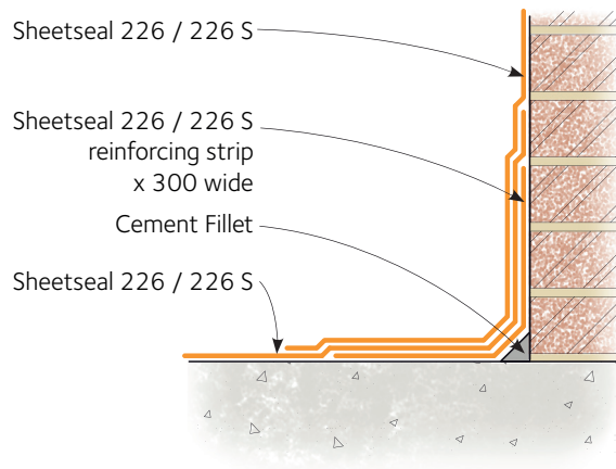
Detail 5 - Internal angle
