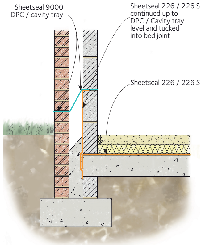
Detail 3 - Ground Floor DPM
