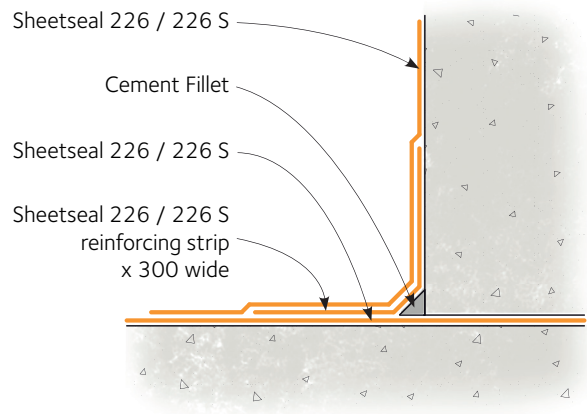
Detail 4 - External Continuity detail
