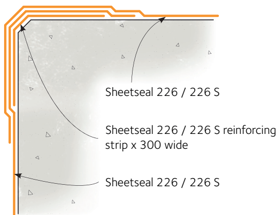
Detail 6 - External angle
