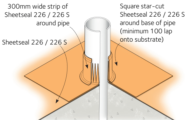
Detail 8 - Pipe Service entry
