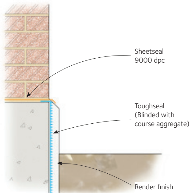
Plinth detail
