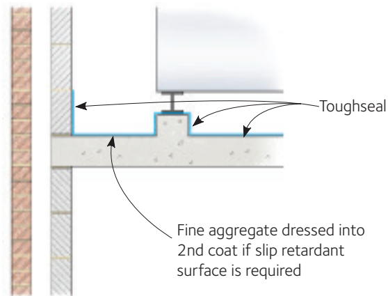
Detail 1 - Plant room detail, horizontal wearing surface
