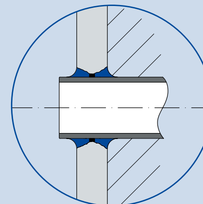
Pipe Inlet
